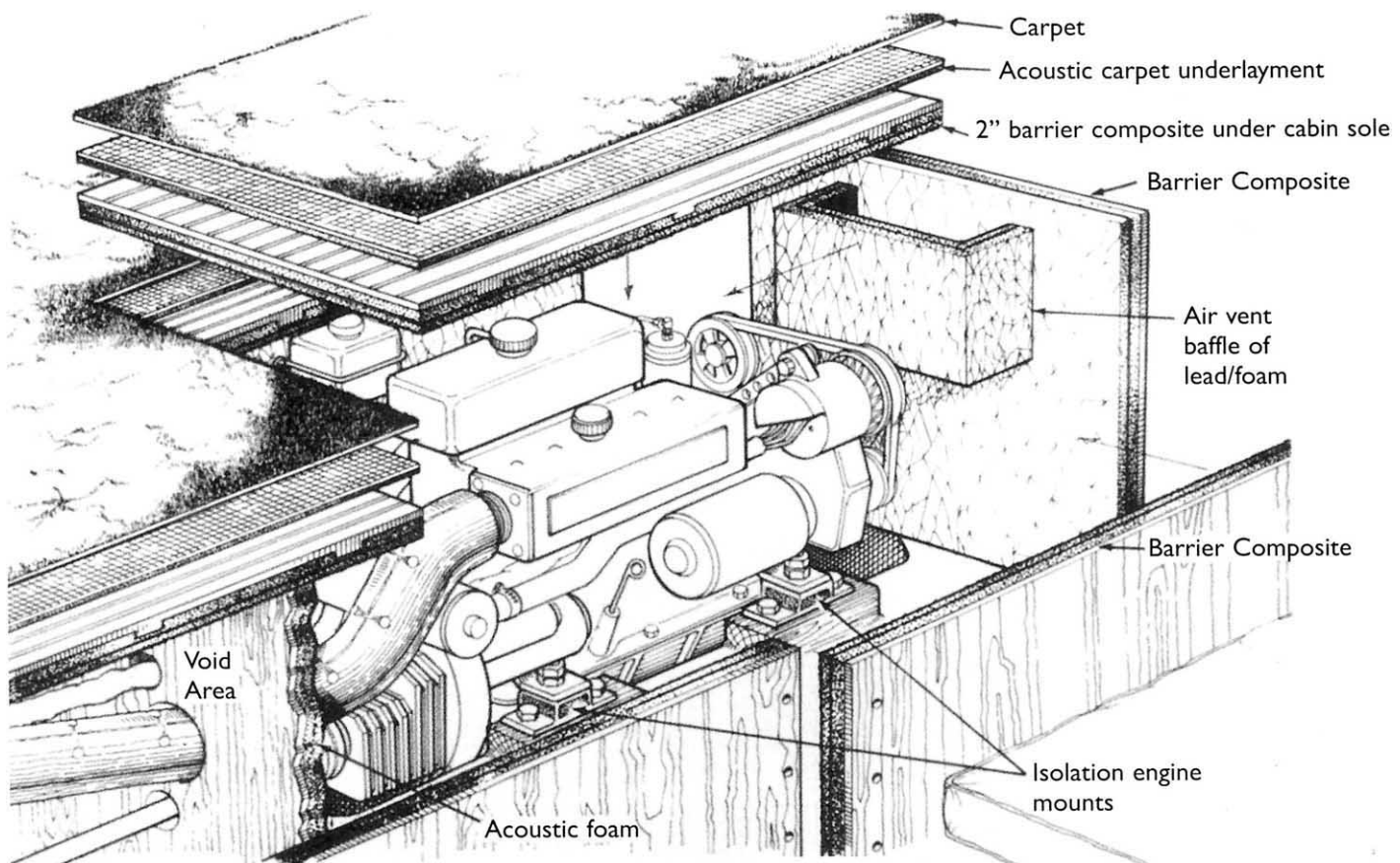
Typical Engine Compartment Insulation—Small to Midsize Boat
